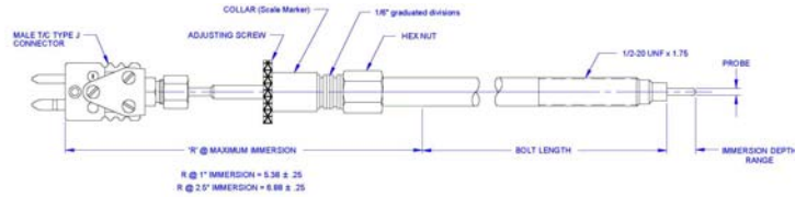
Figure 2. Dimensional Assembly
